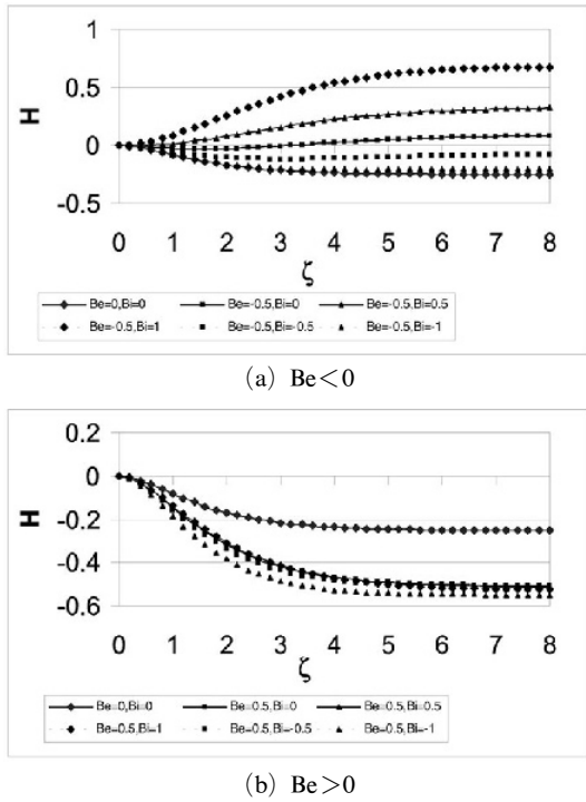
Fig. 3 Steady state profile of the vertical velocity component H for various values of the Hall parameter Be and the ion slip parameter Bi
